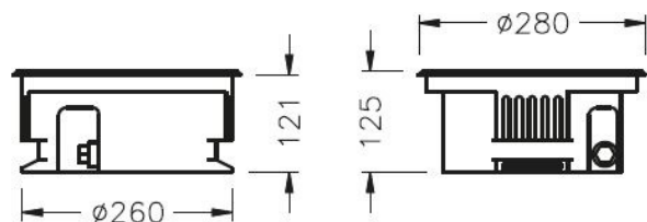
UPLIGHT 280
