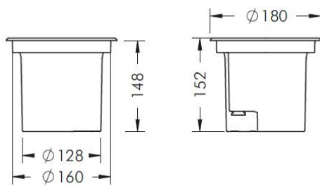
UPLIGHT 180
