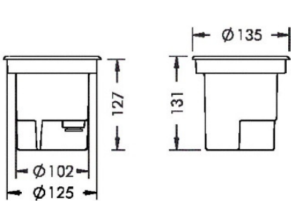
UPLIGHT 135
