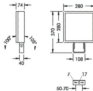
SUPERLIGHT LED 3
