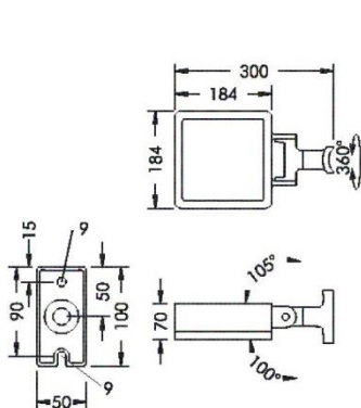
SUPERLIGHT LED 1
