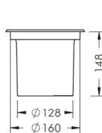
UPLIGHT 180
