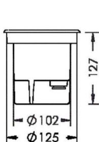
UPLIGHT 135
