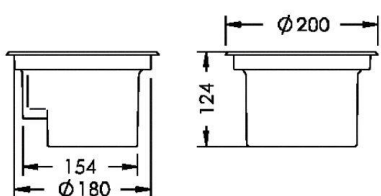
UPLIGHT 200
