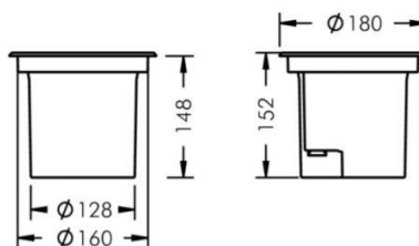
UPLIGHT 180
