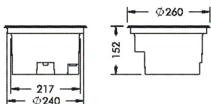
UPLIGHT 260
