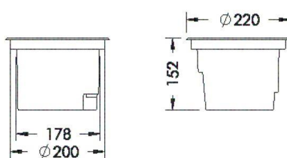
UPLIGHT 220
