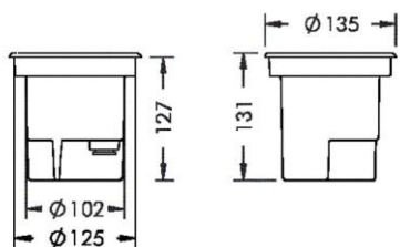
UPLIGHT 135
