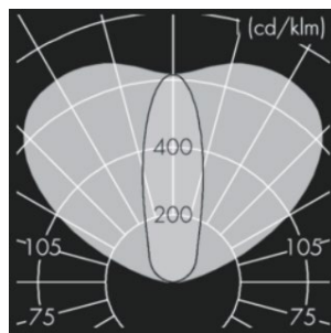
WALL WASHER
