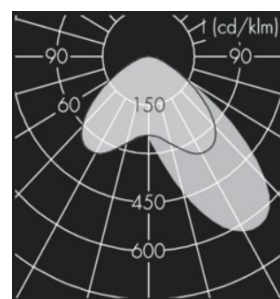
ASYMMETRISK
