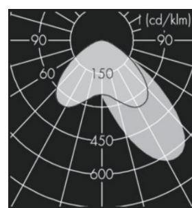
ASYMMETRISK
