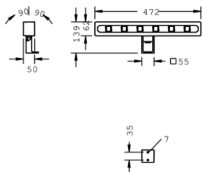
STANDARD
