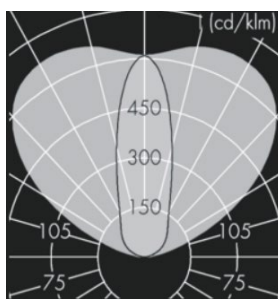
WALL WASHER
